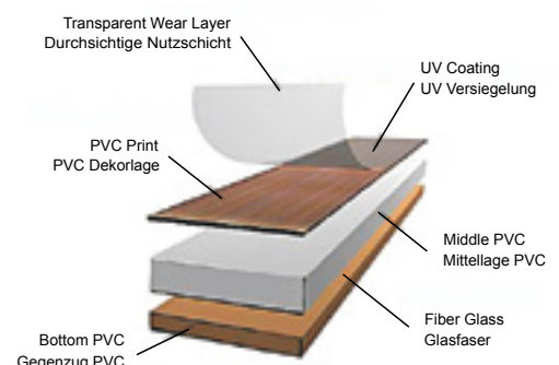
Aufbau LSC + LSL Diele Structure LSC + LSL Plank 2.0/0.3 + 4.0/0.3mm
